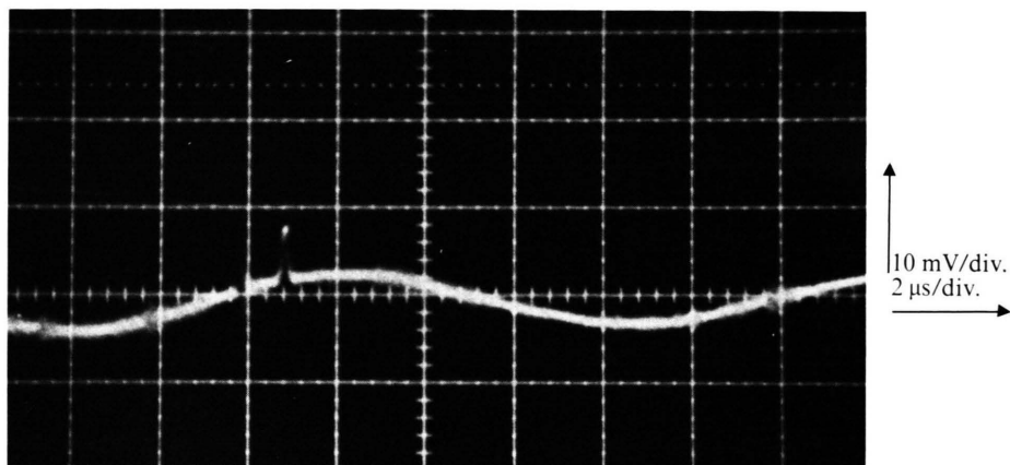
Fig. 1. Registration of the photomultiplier in case of a pure Li wire. The upward deflection is the timing pulse.
